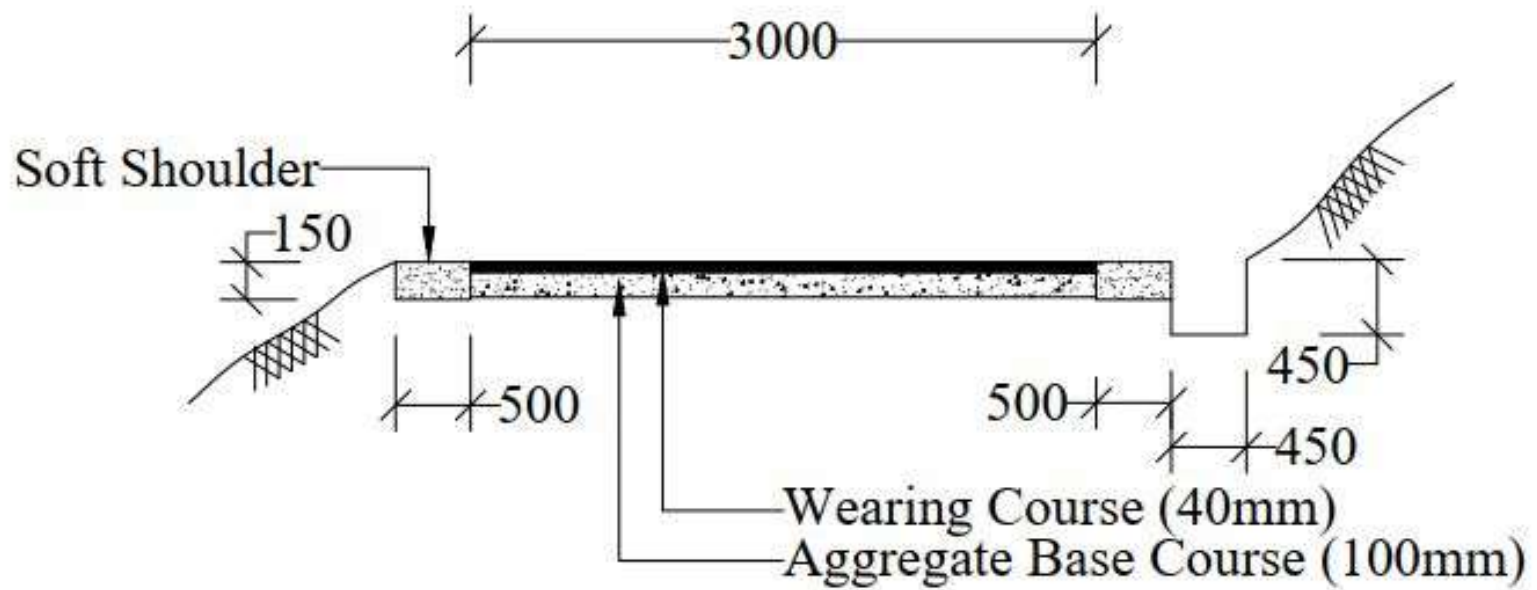
CROSS SECTION FOR EXISTING MACADAM RURAL ROADS (CARRIAGEWAY WIDTH 3.0m)
